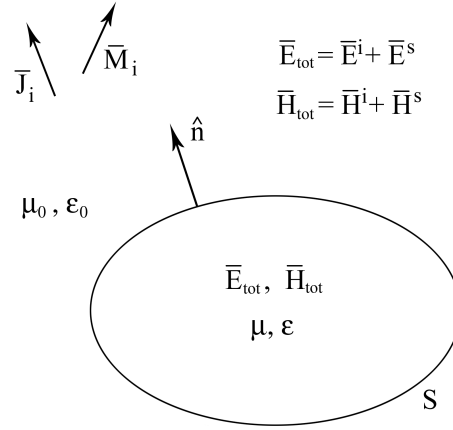
Figure 37. The scattering problem (reproduced from [13]). The object is depicted by the surface S with normal unit vector \hat{n} . The total fields \vec{E}_{tot} and \vec{H}_{tot} are made up of the incident and scattered fields. \vec{J}_i and \vec{M}_i are the sources of the incident field. The parameters of the scattering object and the surrounding free space are \mu, \epsilon and \mu_0, \epsilon_0 , respectively.
